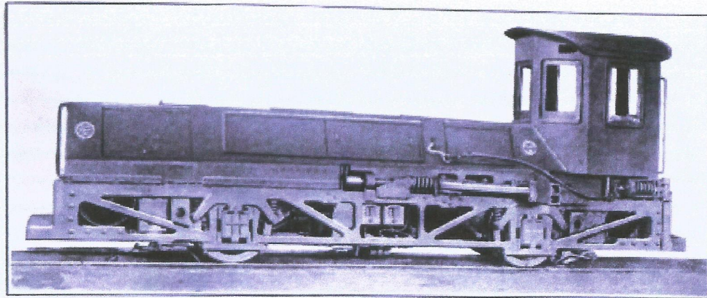
25-Ton Push-Pole Locomotive of the Pennsylvania Railroad
